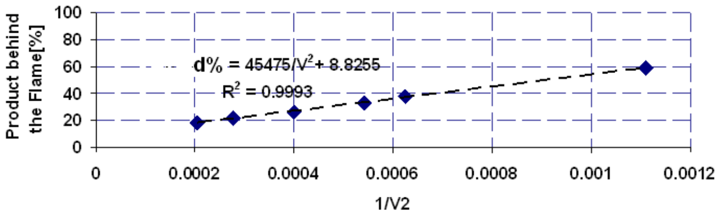
Fig. 4-35. Product density & speed of flame front
