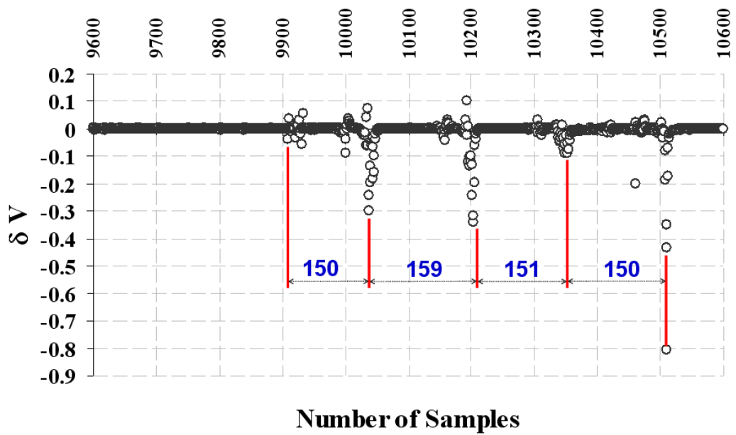
Fig. 2-5. Voltage difference using data in Fig. 4 for layered Al/CuO nano thin film deposited on a substrate
