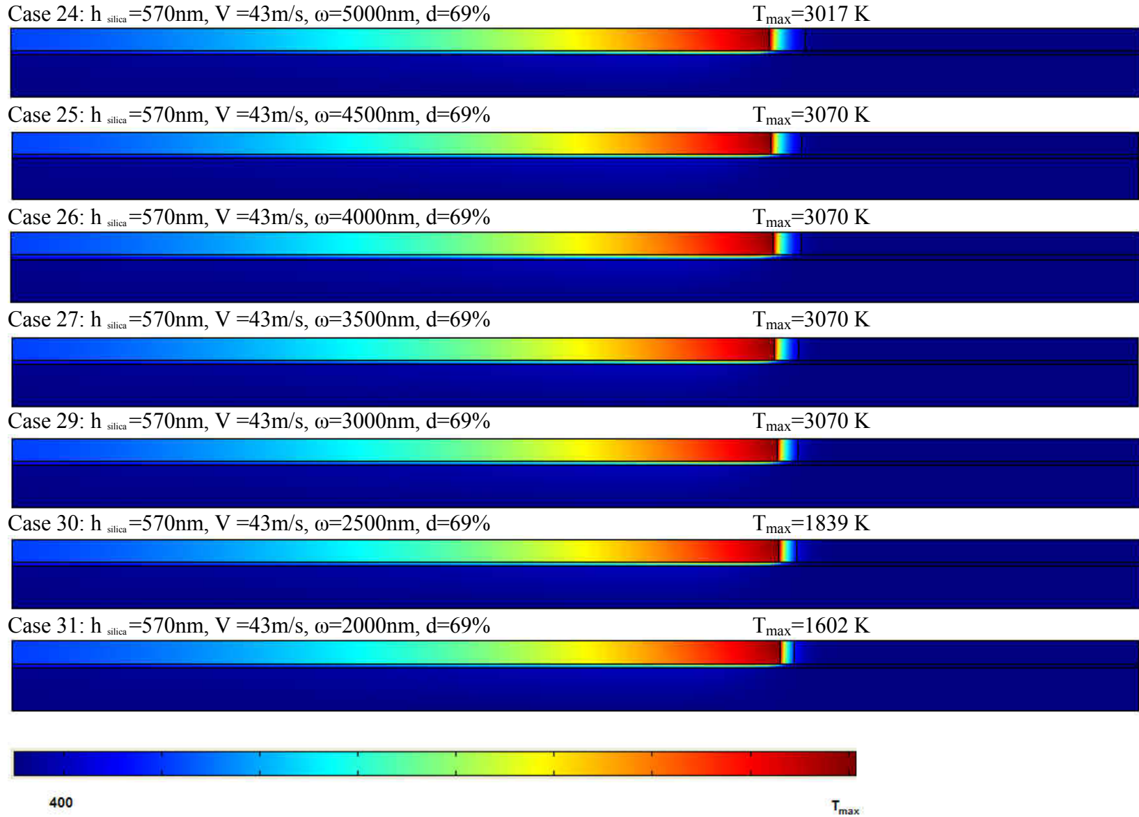
Fig. 4-18. Temperature profile at the interface of thin film and silica substrate
